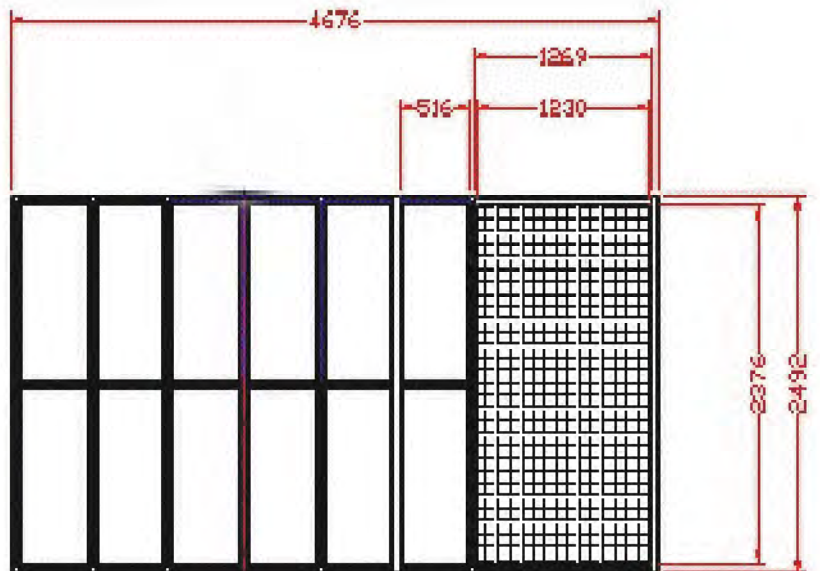
Single heating collector (right or left alignment) with 1kWp PV
